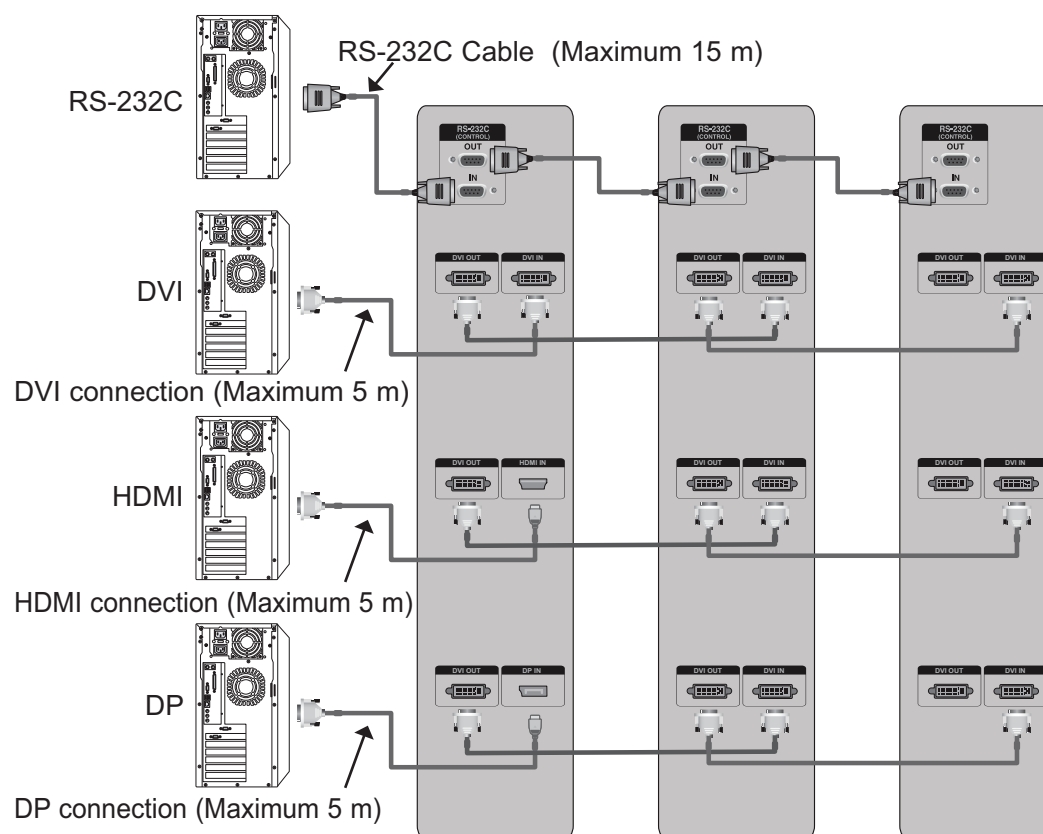
BACK PANEL
